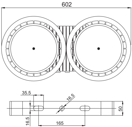
Installation Dimension
