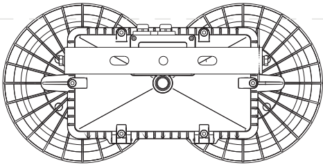
Installation Dimension
