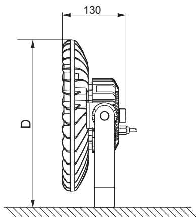
Seat mounting
