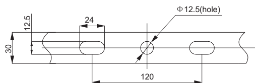
Installation dimensions
